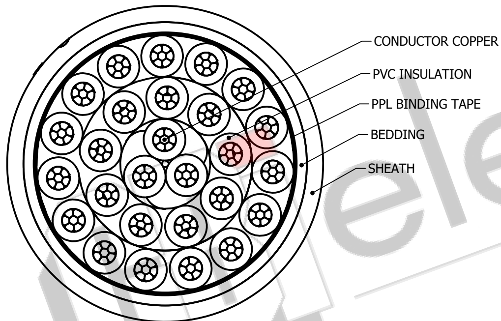
SECTIONAL VIEW
