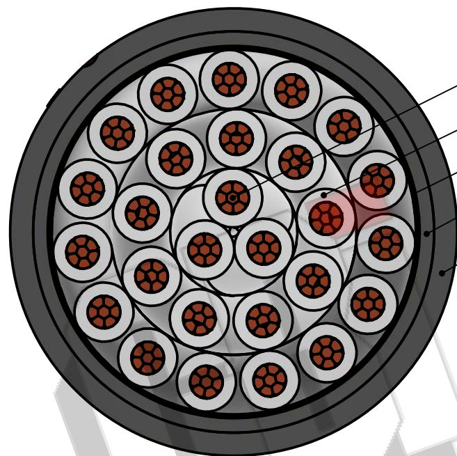
SECTIONAL VIEW
