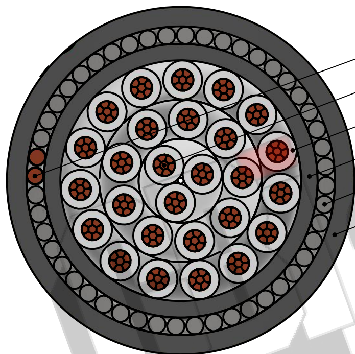
SECTIONAL VIEW
