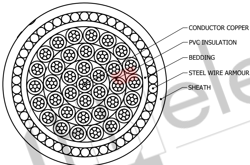
SECTIONAL VIEW
