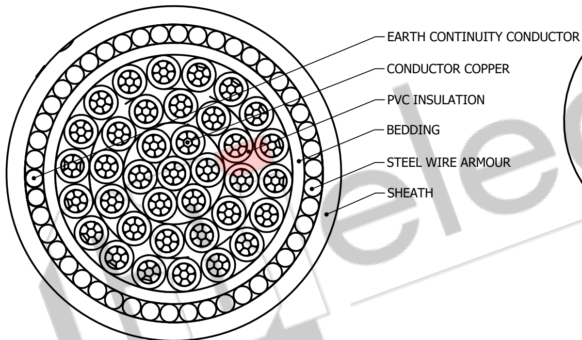
SECTIONAL VIEW
