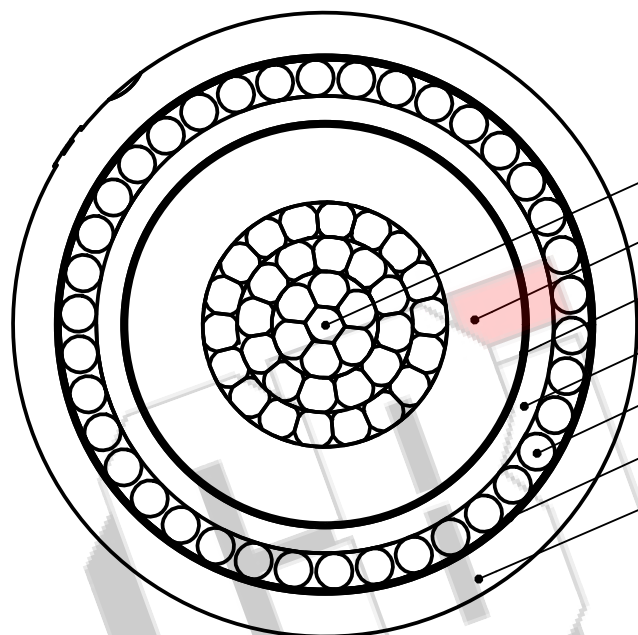
SECTIONAL VIEW
