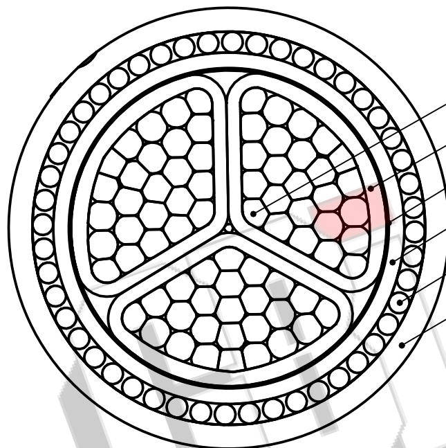
SECTIONAL VIEW
