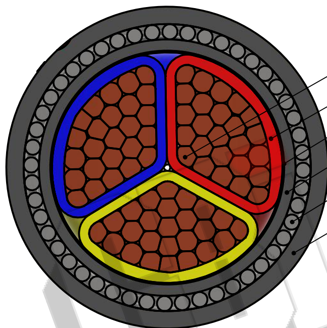
SECTIONAL VIEW
