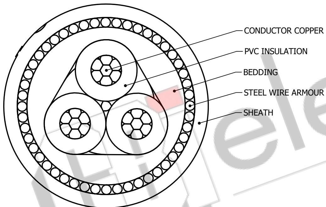
SECTIONAL VIEW
