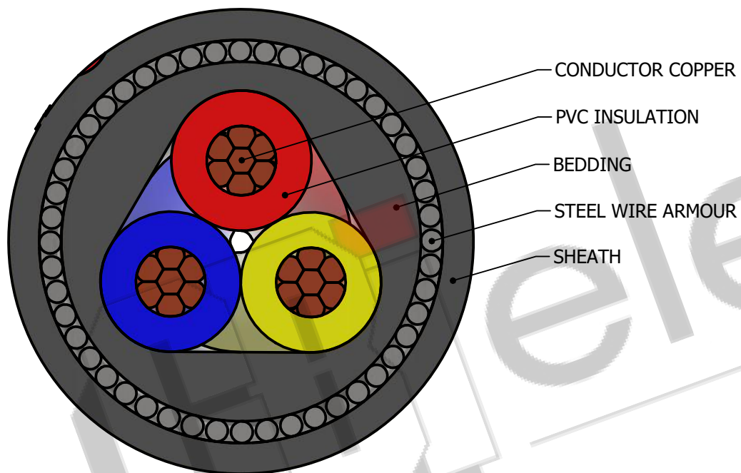
SECTIONAL VIEW
