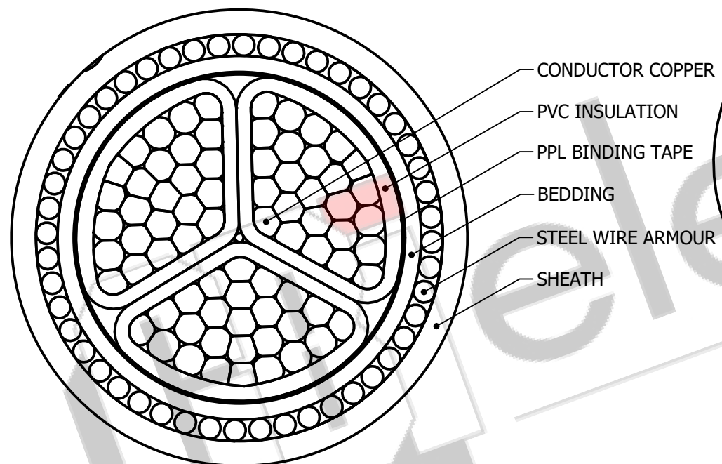
SECTIONAL VIEW
