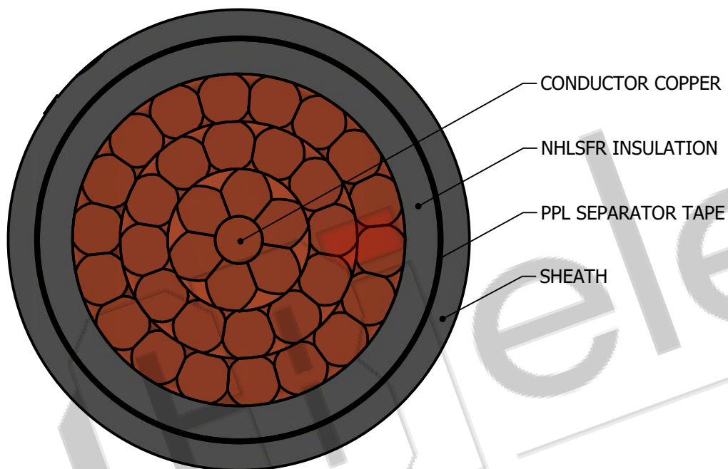
SECTIONAL VIEW
