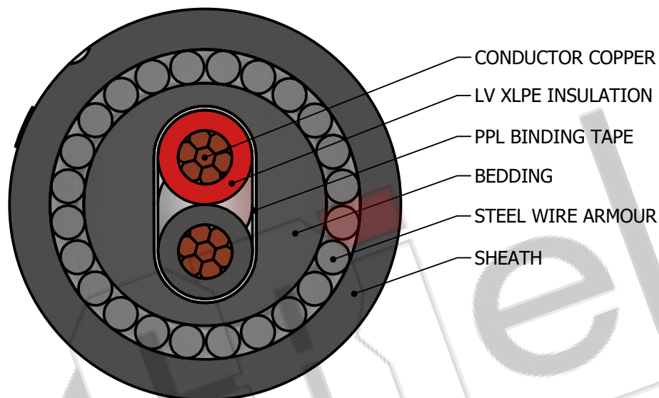
SECTIONAL VIEW
