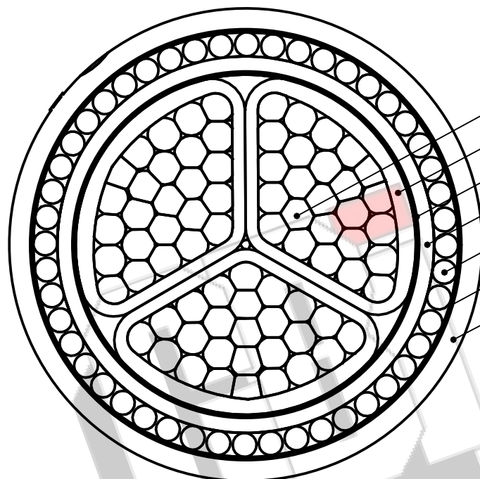
SECTIONAL VIEW
