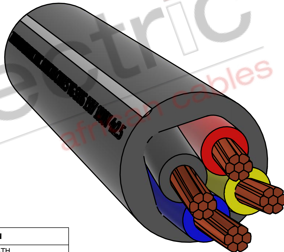
ISOMETRIC VIEW
