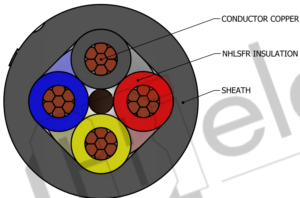
SECTIONAL VIEW
