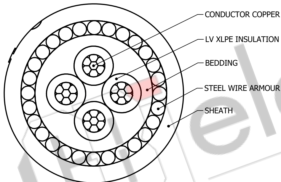
SECTIONAL VIEW
