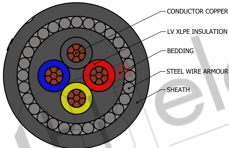
SECTIONAL VIEW
