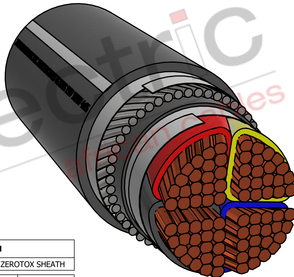
ISOMETRIC VIEW
