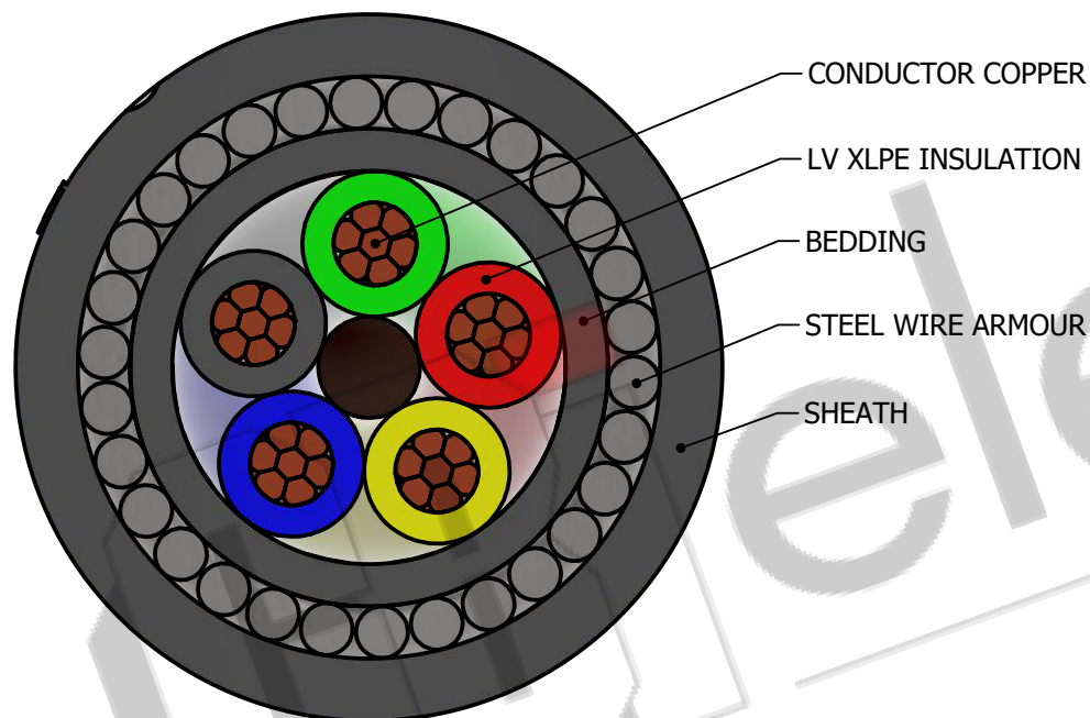
SECTIONAL VIEW
