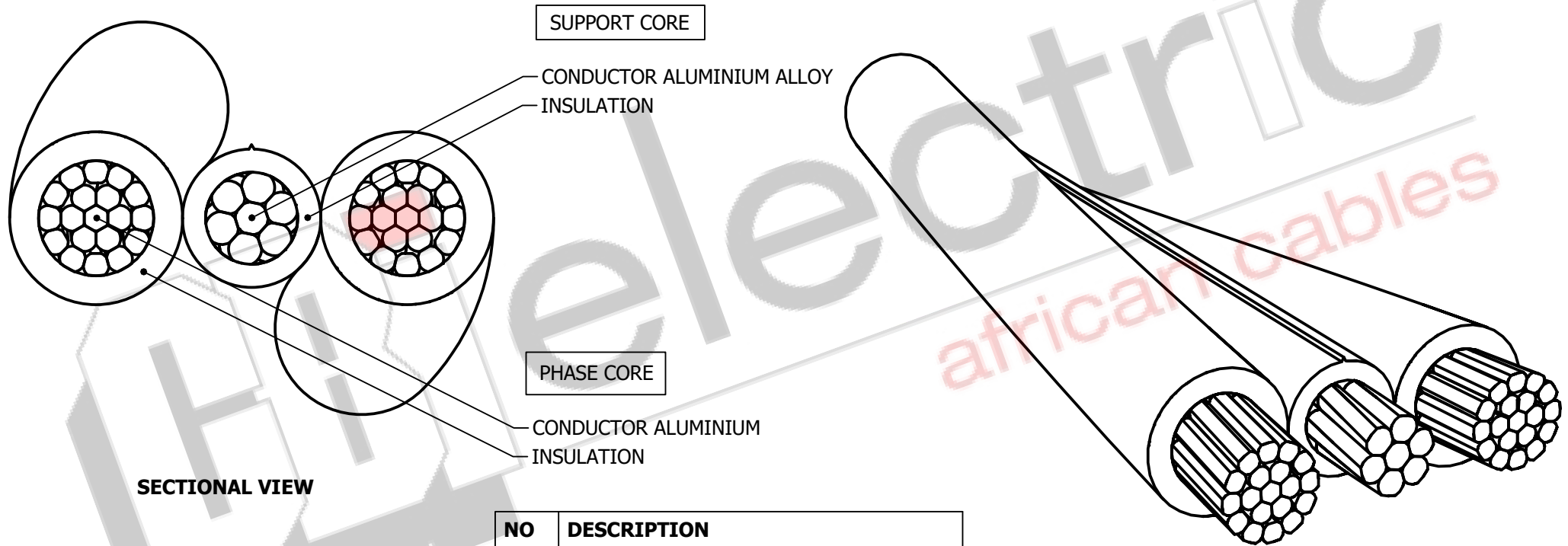
ISOMETRIC VIEW
