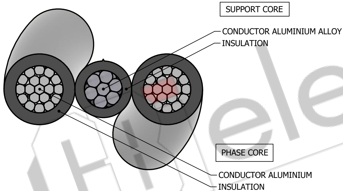
SECTIONAL VIEW
