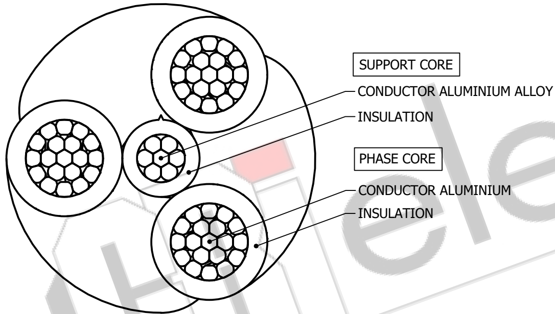
SECTIONAL VIEW
