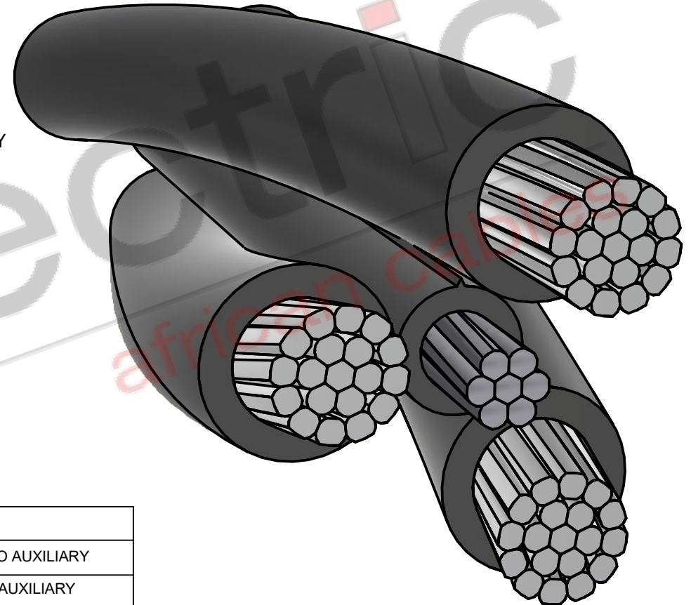
ISOMETRIC VIEW
