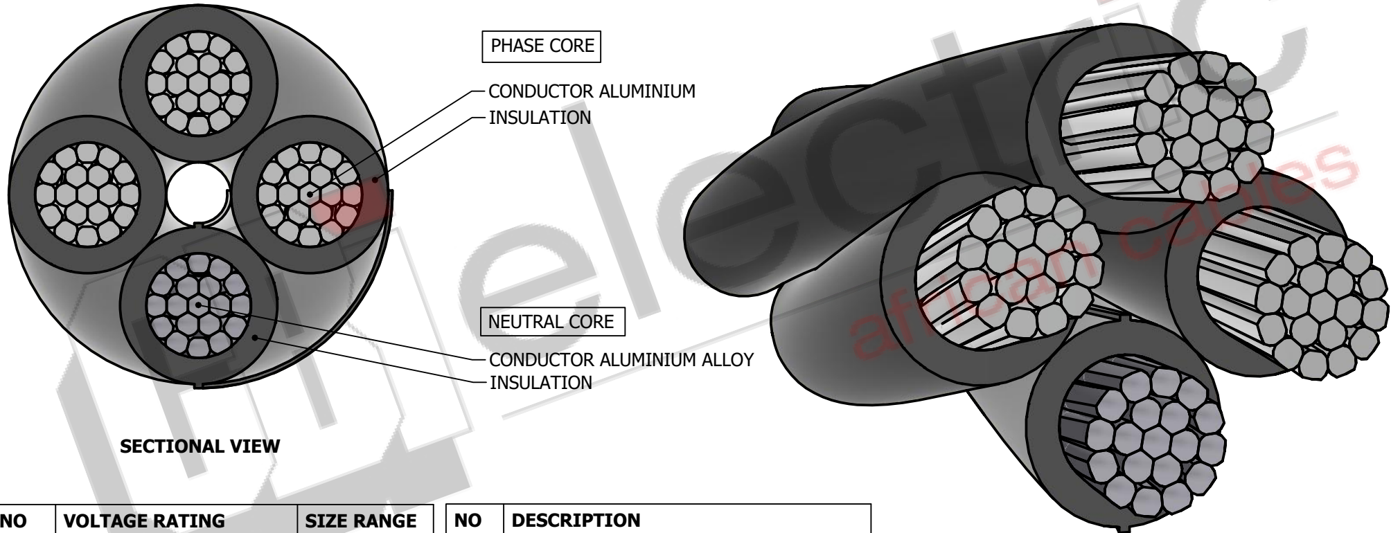
ISOMETRIC VIEW
